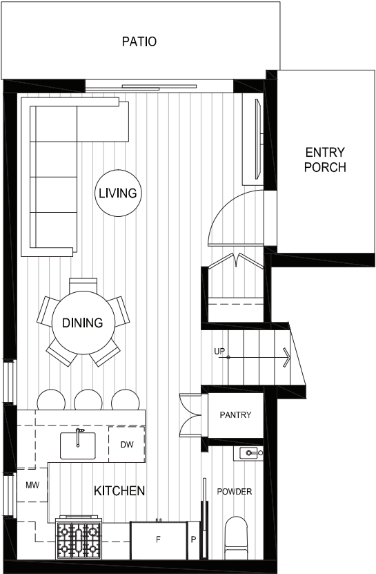
MAIN 551 sq ft
